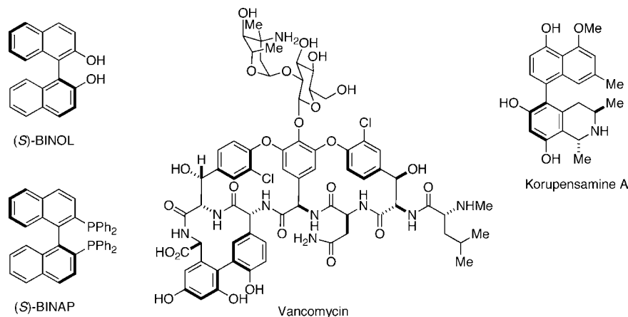
Figure 1. Ligands and biologically active natural products containing the axially chiral biaryl structural motif.
