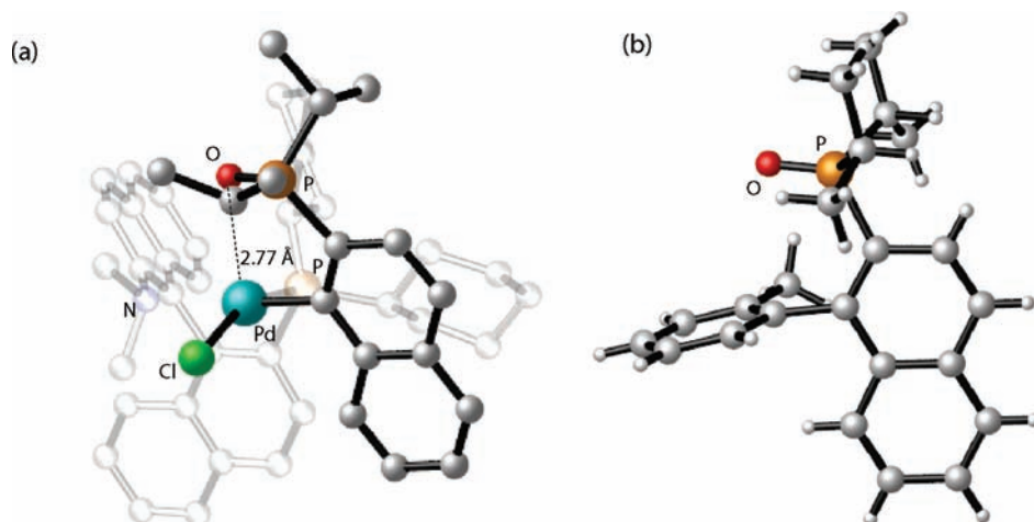
Figure 3. Crystallographic structures for the (a) oxidative addition complex of Pd(KenPhos) with (1-chloro-2-naphthyl)diisopropylphosphine oxide. (Hydrogen atoms have been omitted and atoms belonging to the KenPhos ligand have been faded for clarity.) (b) Coupled biaryl product from the reaction of (1-chloro-2-naphthyl)diisopropylphosphine oxide and o -tolylboronic acid.
